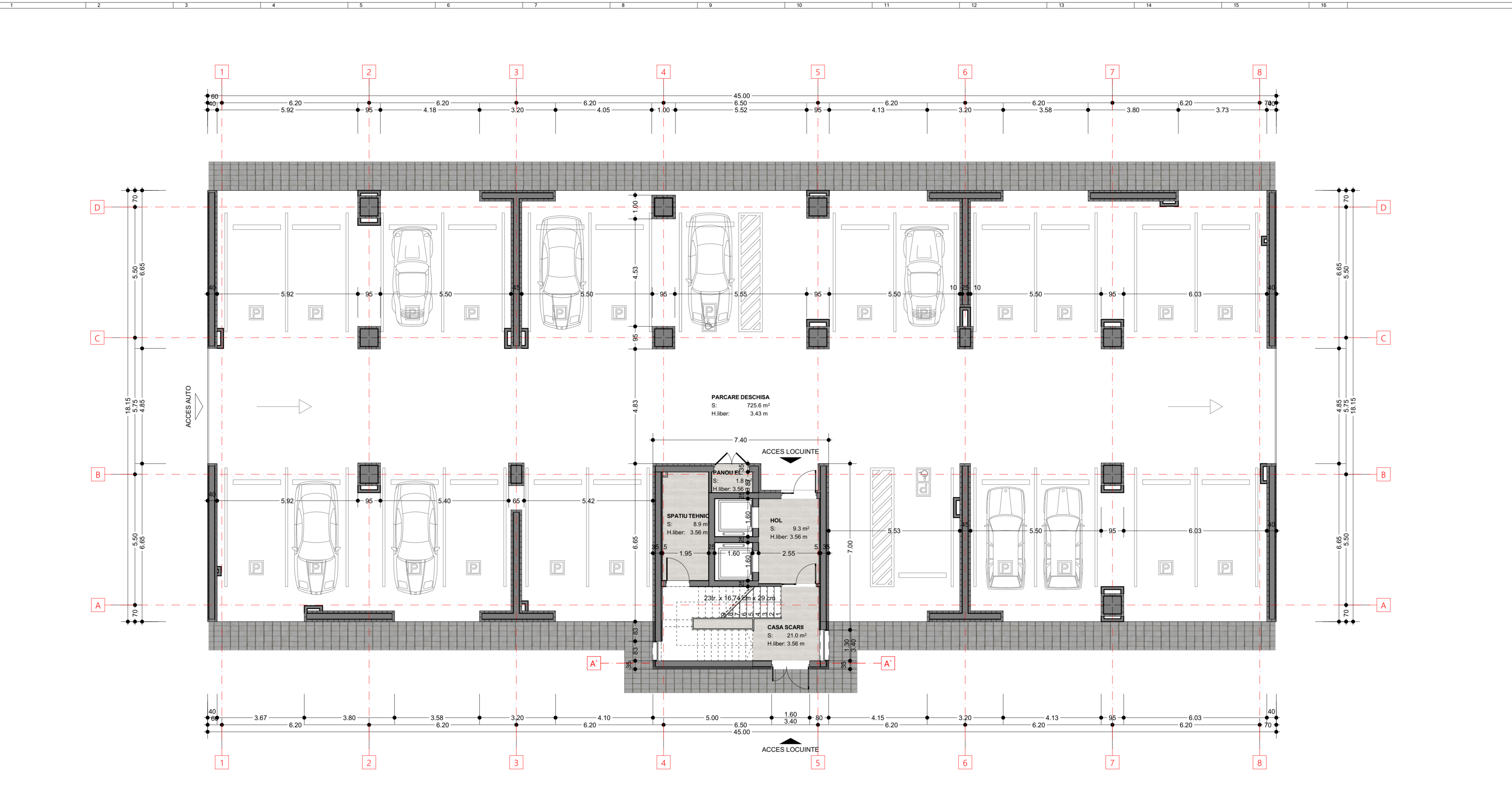
Plan PARTER - tronson B SCARA 1:100
